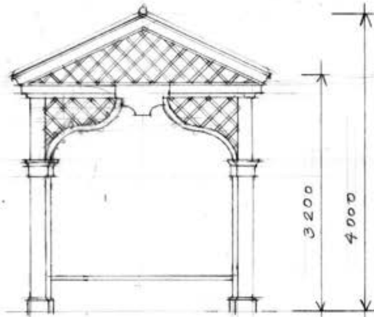
South Elevation
